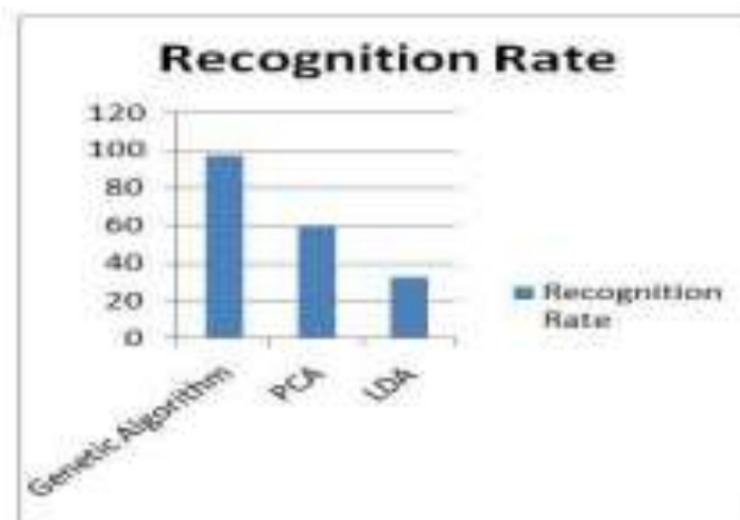
Fig. 4. Recognition rate for ORL database
